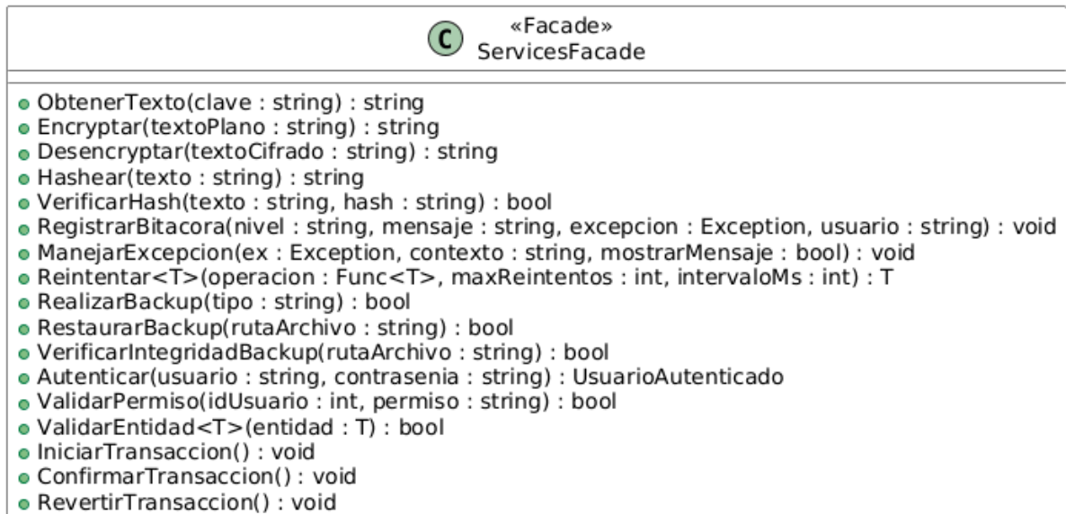
Services - Diagrama de Clases Global - Facade
